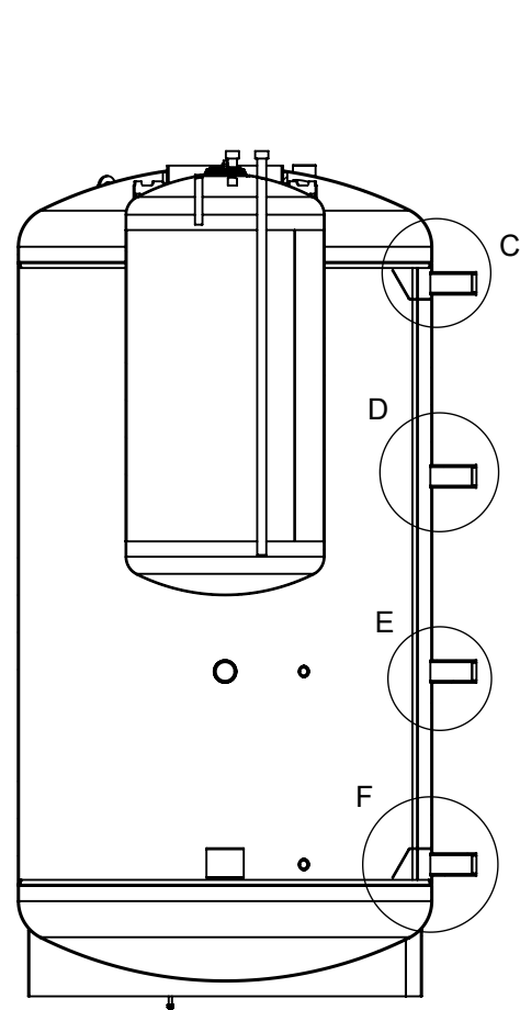
SECTION B-B
