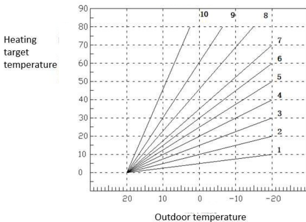
Compensation curve (offset =0)
